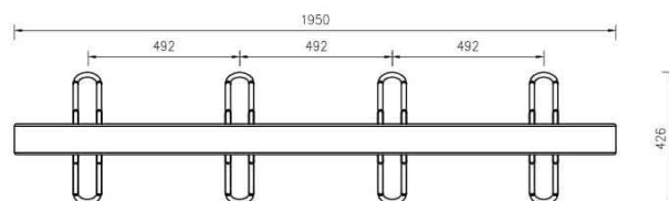
RZUT STOJAKA NA ROWERY
